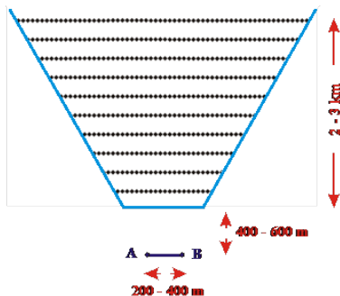
Working area in the RMT-CS method
