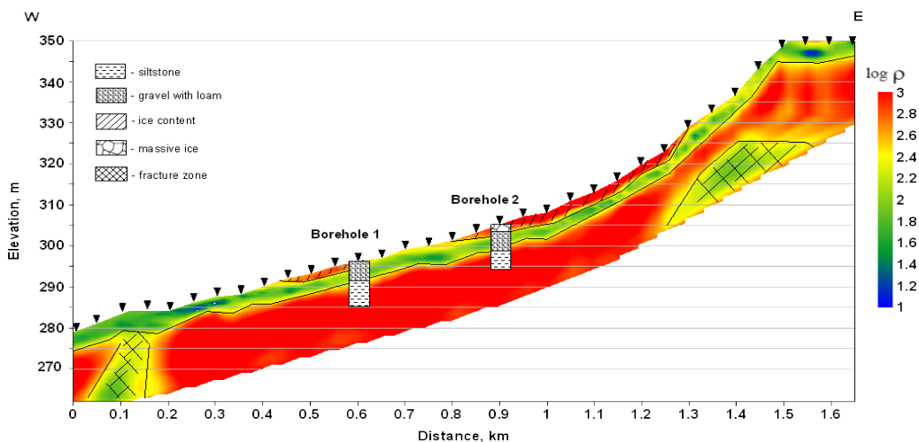
Geoelectric section according to the 2D inversion of CSRMT data (10-1000 kHz) and its comparison with boreholes data, obtained after RMT-CS investigations. Ratio of horizontal and vertical scales is 10:1.
