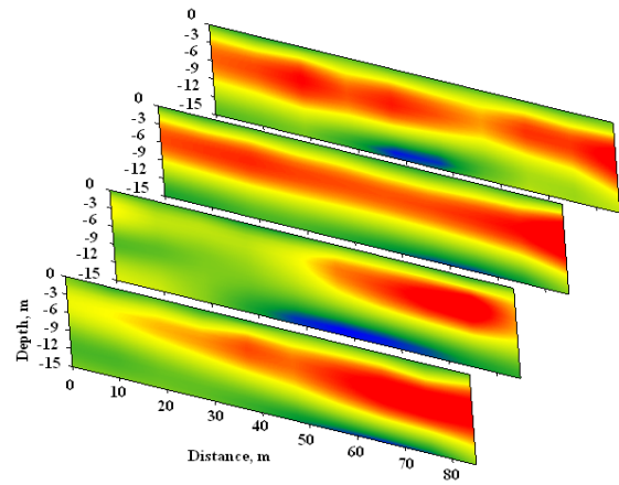
Examples of RMT-CS geoelectric sections
