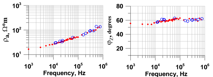
Example of RMT-CS (red) and RMT (blue) sounding curves at 1 km away from the CS.
