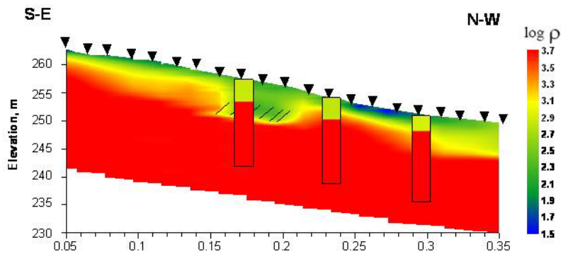
Comparison of CSRMT 2D inversion results (geoelectric section) with 1D VES inversion (columns). Fractured zone is shown by hatching.
