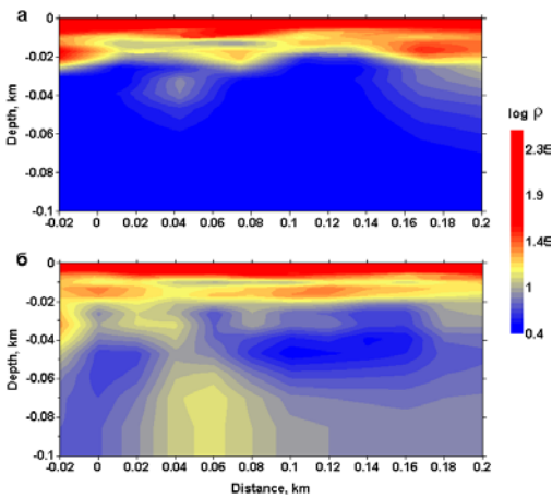
Comparison of 2D inversion results of the RMT method in 12-1000 kHz range (a) and the RMT-CS method in 1-1000 kHz range (b).
