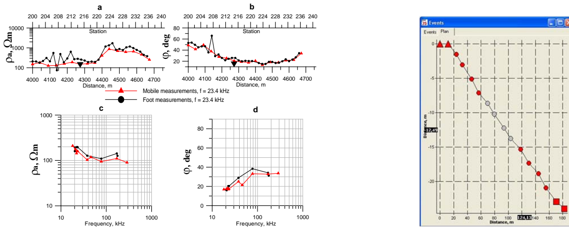
Comparison of the foot (black) and mobile (red) variants of the RMT method on one frequency at measurements along a profile (a, b) and soundings curves at one station (c, d).
