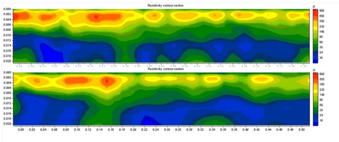
Comparison of results of 2D inversion along a profile of 500 m length (up to the depth of 20 m) on data of foot (above) and mobile (below) measurements by the RMT method.
